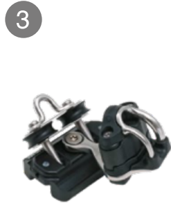
Main car, pivoting sheaves, cam cleat
