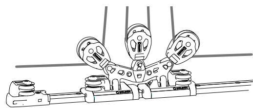
Triple main system
