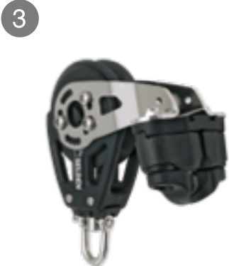
Single swivel/fixed cam
