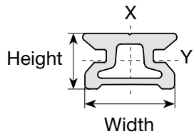
TRACK Standard 22, 30, 42
