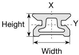
TRACK Pinstop 22, 30, 42
